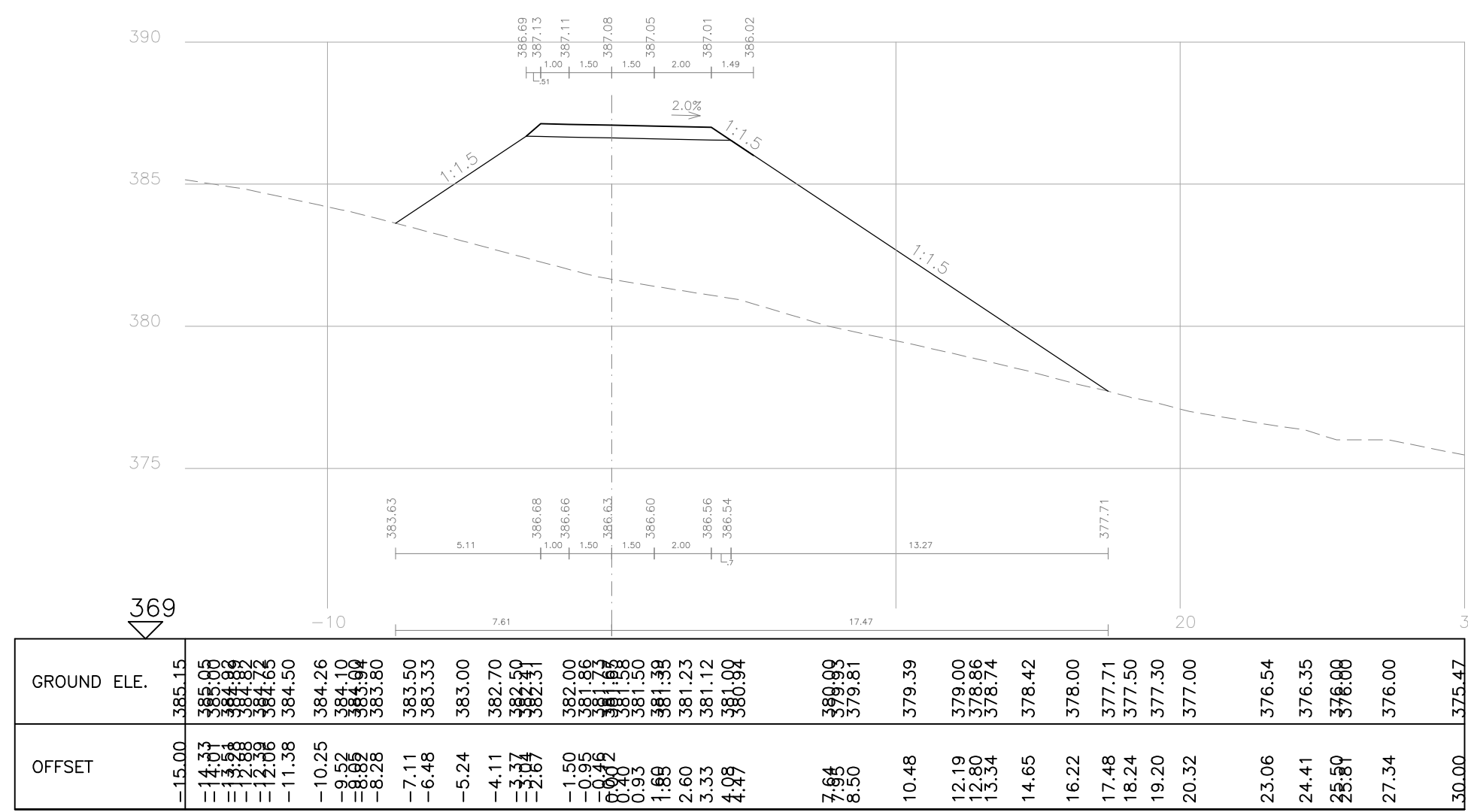
SECTION 217 St. 340 road2
