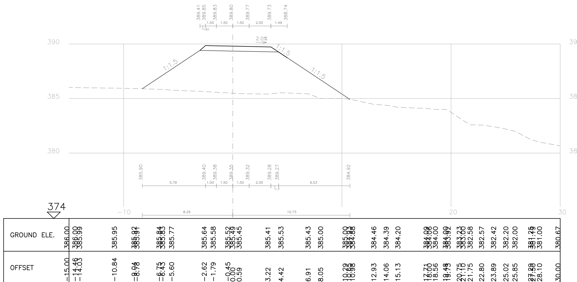
SECTION 221 St. 413.72 road2
