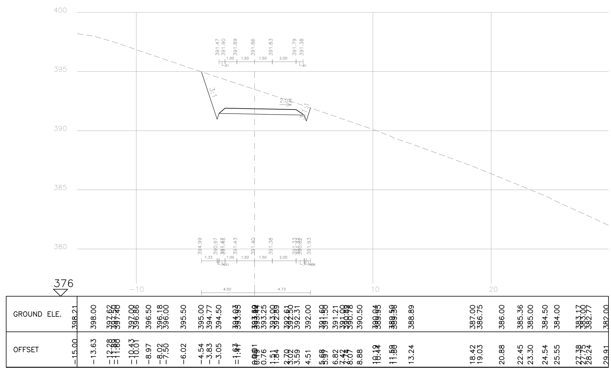
SECTION 215 St. 300 road2
