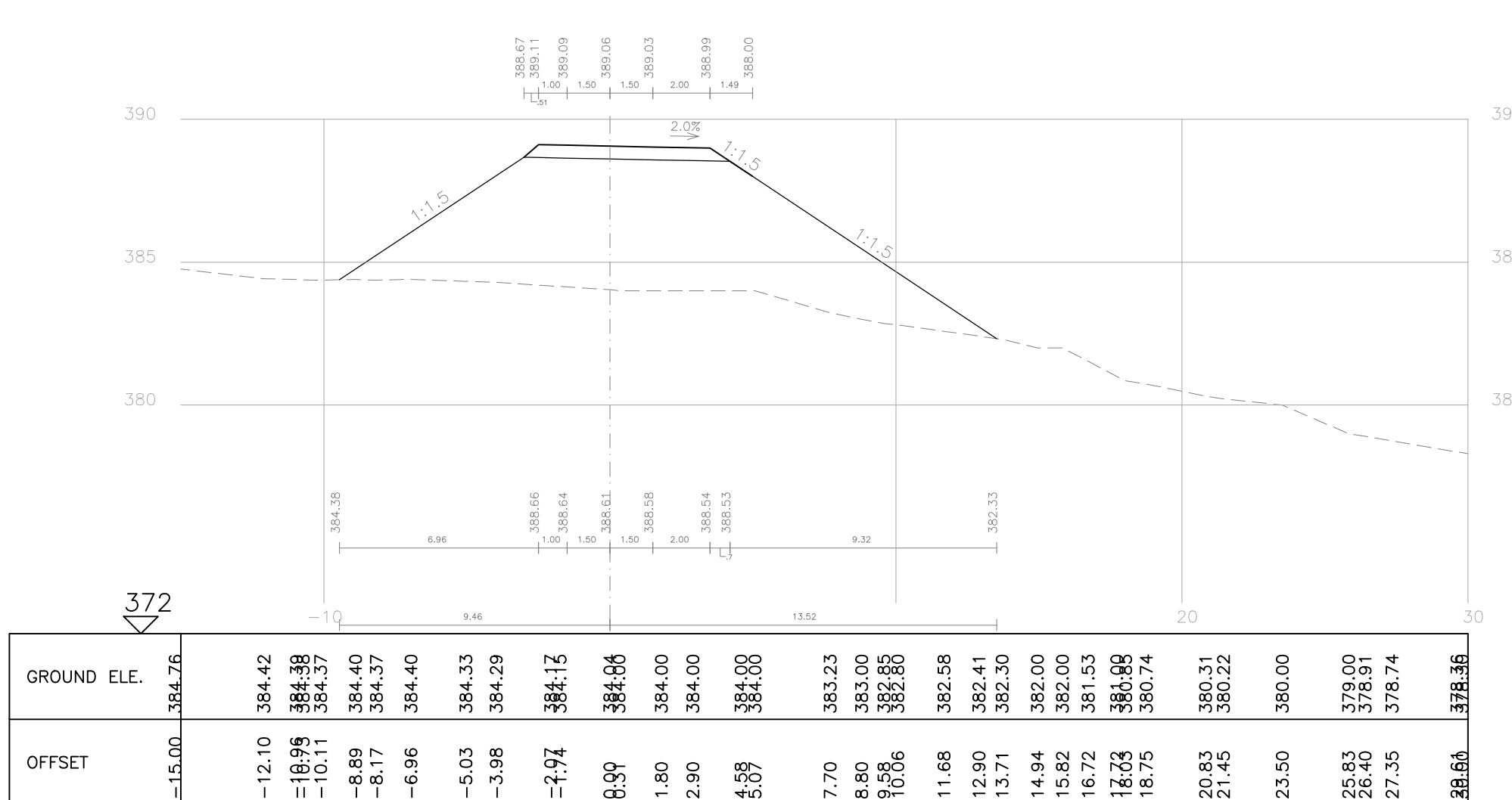
SECTION 220 St. 400 road2
