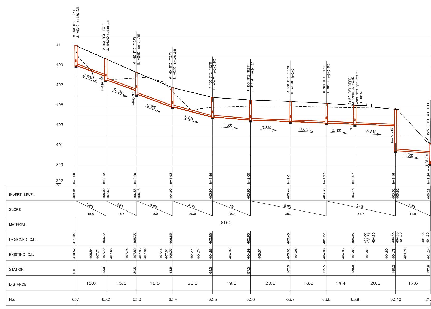
Pipeline 25 - 1:100/1:500
