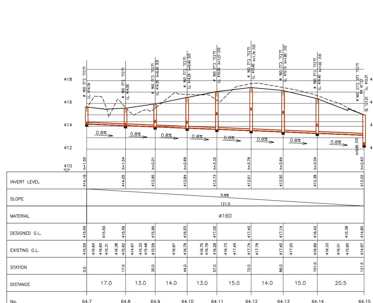
Pipeline 22 - 1:100/1:500
