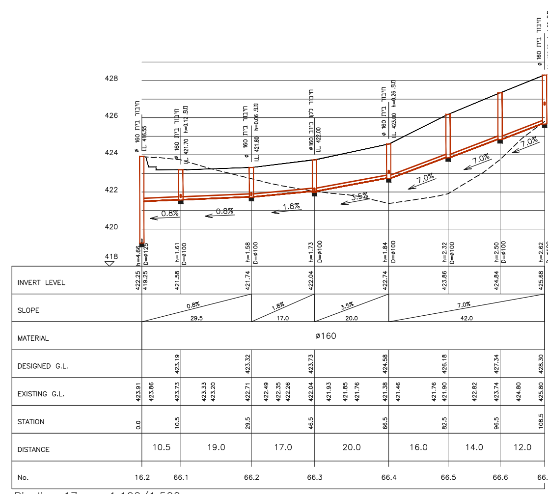
Pipeline 17 = 1:100/1:500
